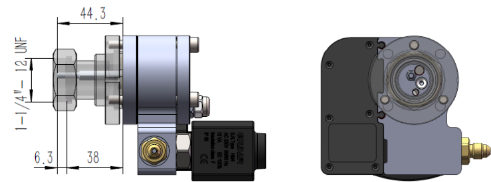
OUT680R-1 带GOA114 旋转锁定适配器与长款喷油管
