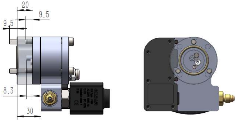
OUT680R-1 带GOA20F 法兰加高块与短款喷油管 OUT680R-1 with GOA20F and short injector pipe
