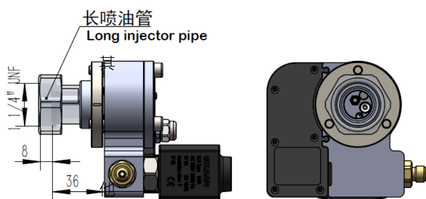
OUT680R-11/114-36 带旋转锁定适配器及长喷油管 OUT680R-11 With GOA114-36 Rotalock Adapter
